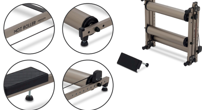
< Roadbike/MTB style > Wheel base size : 1,030mm ver.
